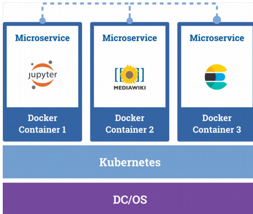
Figure 6.2: Architecture of Remix platform
